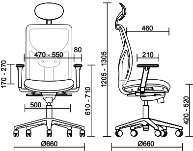
OPERATIVE WITH HEADREST AND 2D ARMRESTS
