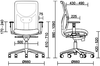
OPERATIVE WITH ARMRESTS ADJUSTABLE IN HEIGHT
