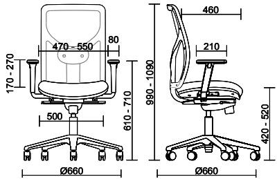
OPERATIVE WITH 2D ARMRESTS
