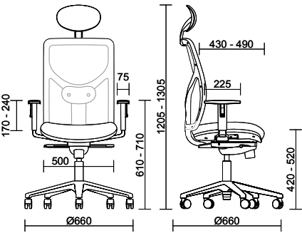
OPERATIVE WITH HEADREST AND ARMRESTS ADJUSTABLE IN HEIGHT
