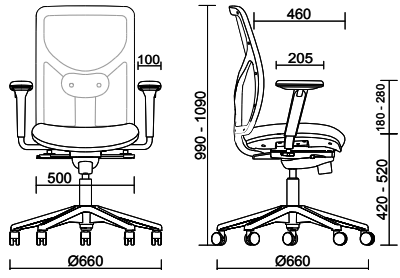
OPERATIVE WITH 4D ARMRESTS
