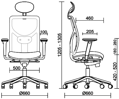
OPERATIVE WITH HEADREST AND 4D ARMRESTS
